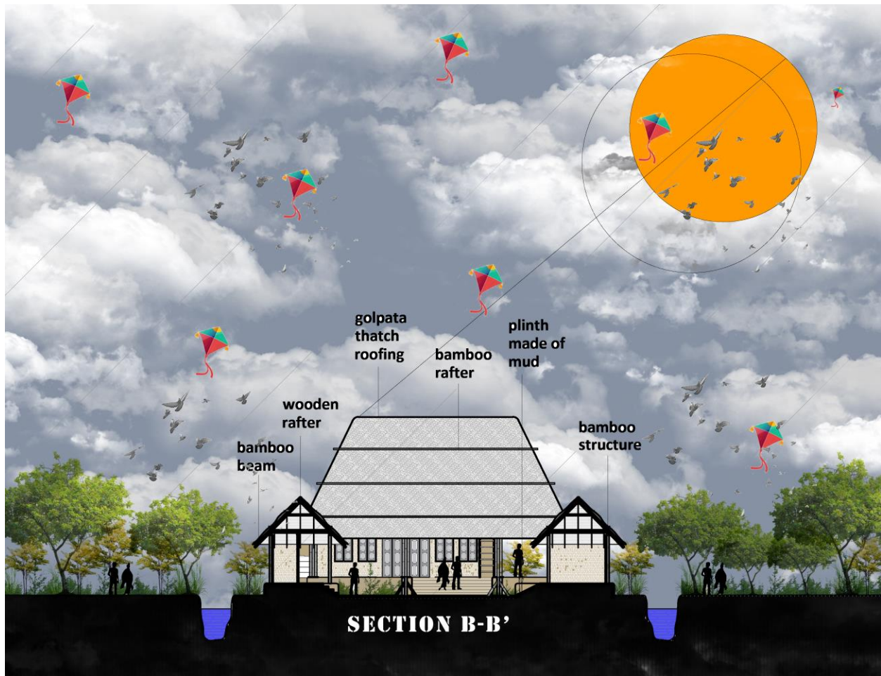
Figure: section bb'
